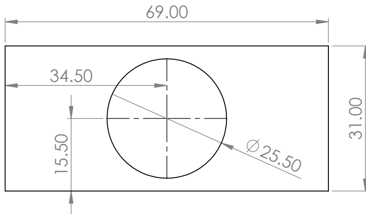
Top (1/2in plywood)
